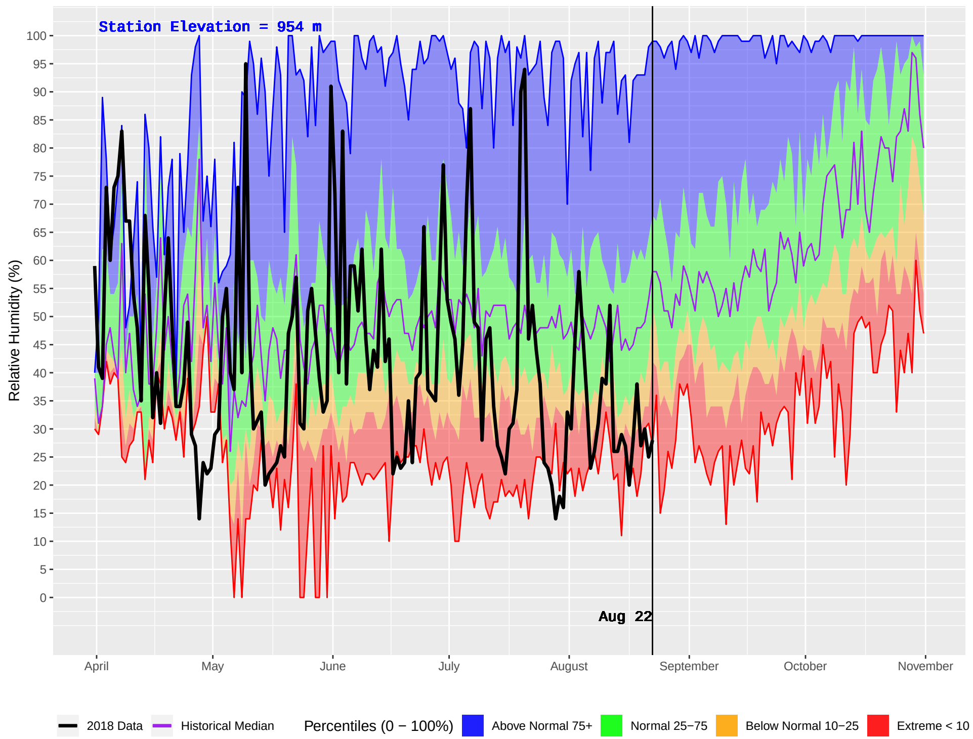
NADINA (179) : Historical (1985–2016) and Current (2018) Daily Relative Humidity
