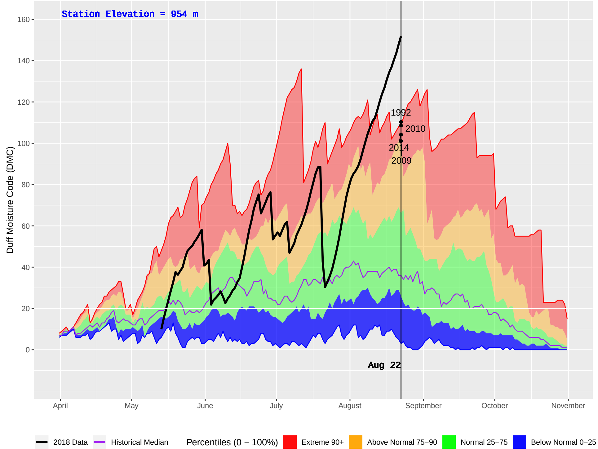
NADINA (179) : Historical (1985–2016) and Current (2018) Daily Duff Moisture Code (DMC)
