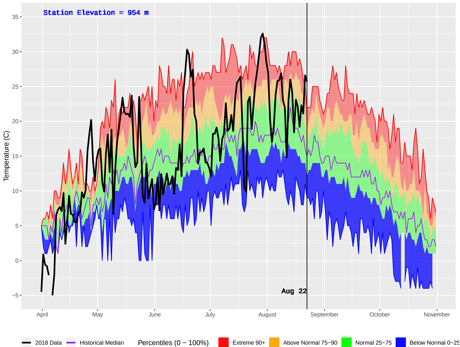
NADINA (179) : Historical (1985–2016) and Current (2018) Daily Temperature
