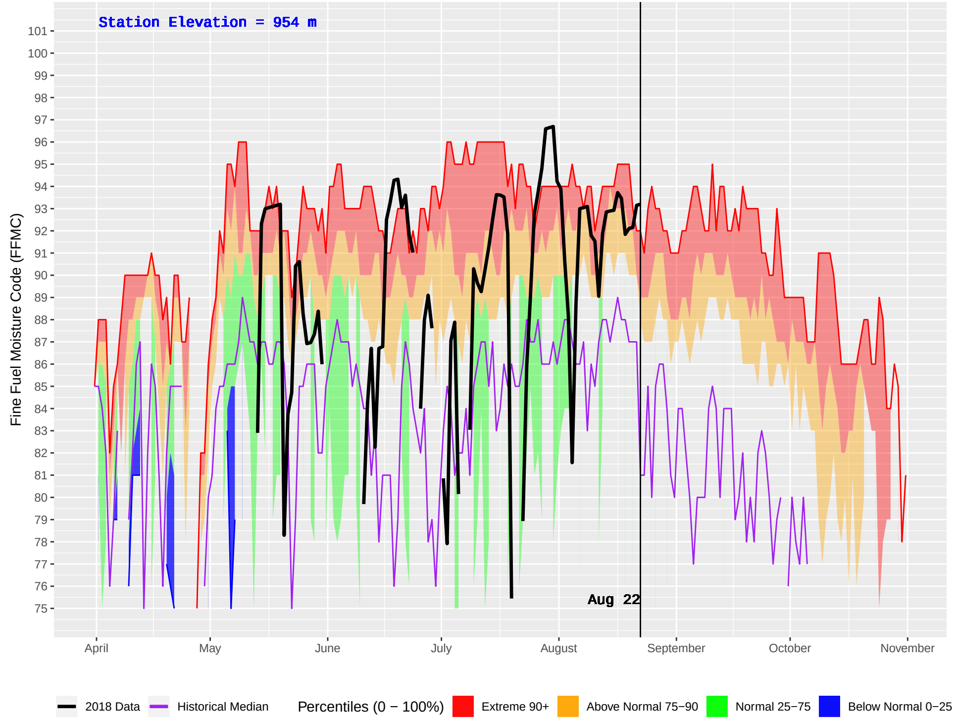
NADINA (179) : Historical (1985–2016) and Current (2018) Daily Fine Fuel Moisture Code (FFMC)
