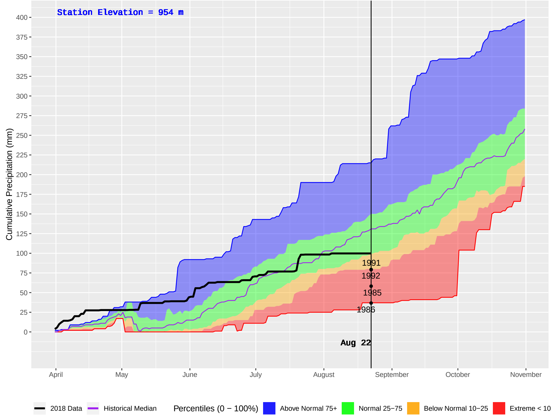
NADINA (179) : Historical (1985–2016) and Current (2018) Daily Cumulative Precipitation
