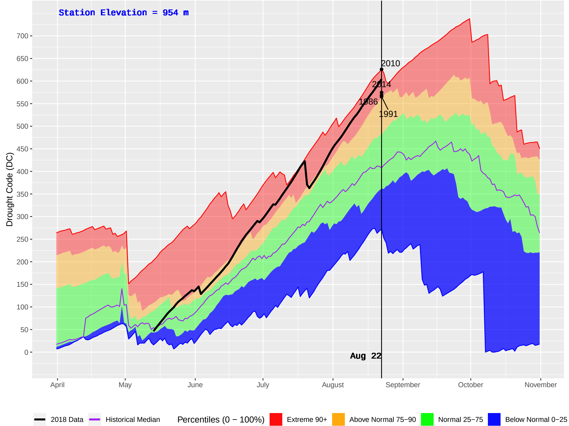
NADINA (179) : Historical (1985–2016) and Current (2018) Daily Drought Code (DC)
