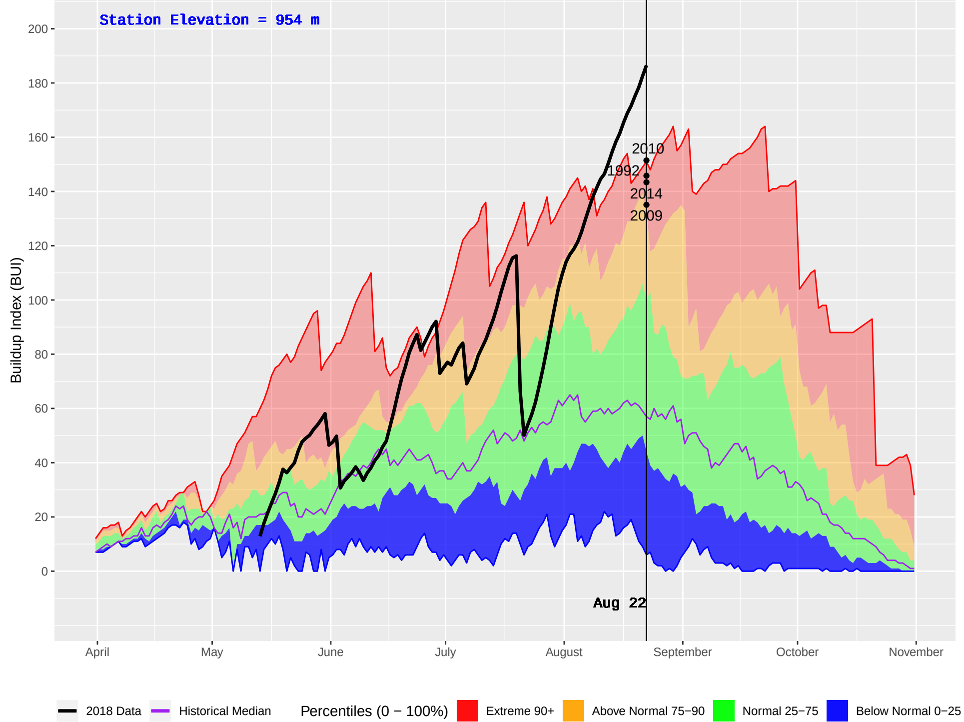
NADINA (179) : Historical (1985–2016) and Current (2018) Daily Buildup Index (BUI)
